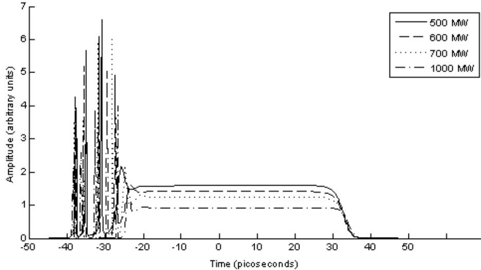
Figure 4.5. Increasing initial peak powers have little effect on the rate that a pulse collapses. After 0.50 meters of propagation, each pulse has collapsed roughly the same amount. However, note that the number of collapse events increases with peak power.
